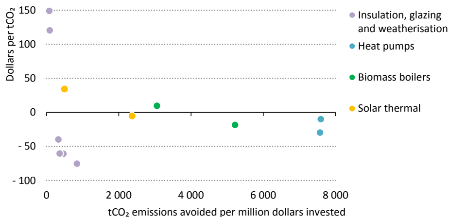
Figure 2.19 ▶ CO 2 emissions abatement costs for space heating and annual avoided emissions by measure per million dollars invested
